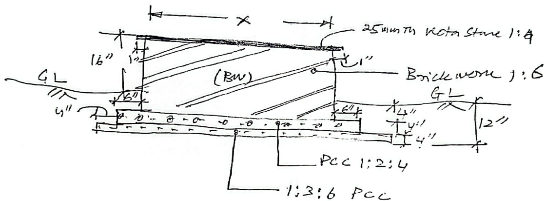
Typ. section of Pedestal
